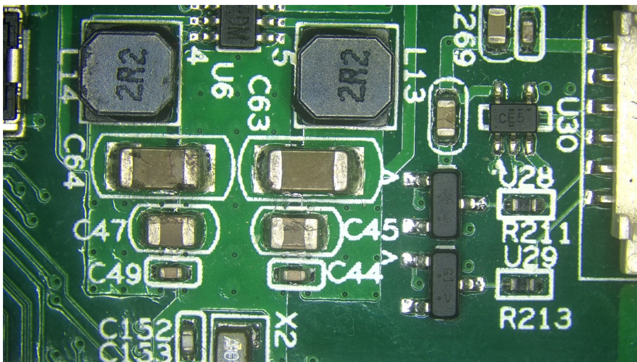
Figure 6-6 Circuit Board Captured with CXCAM4K8MPC
