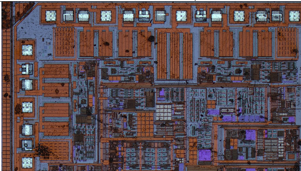
Figure 3-21 Semiconductor Samples Photographed by the OUMIT CX43M Metallographic Microscopy System Captured with X8CAM4K16MPA
