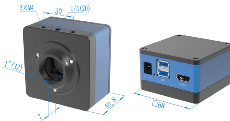
Figure 3-99 Dimension of O5CAM4K Series
