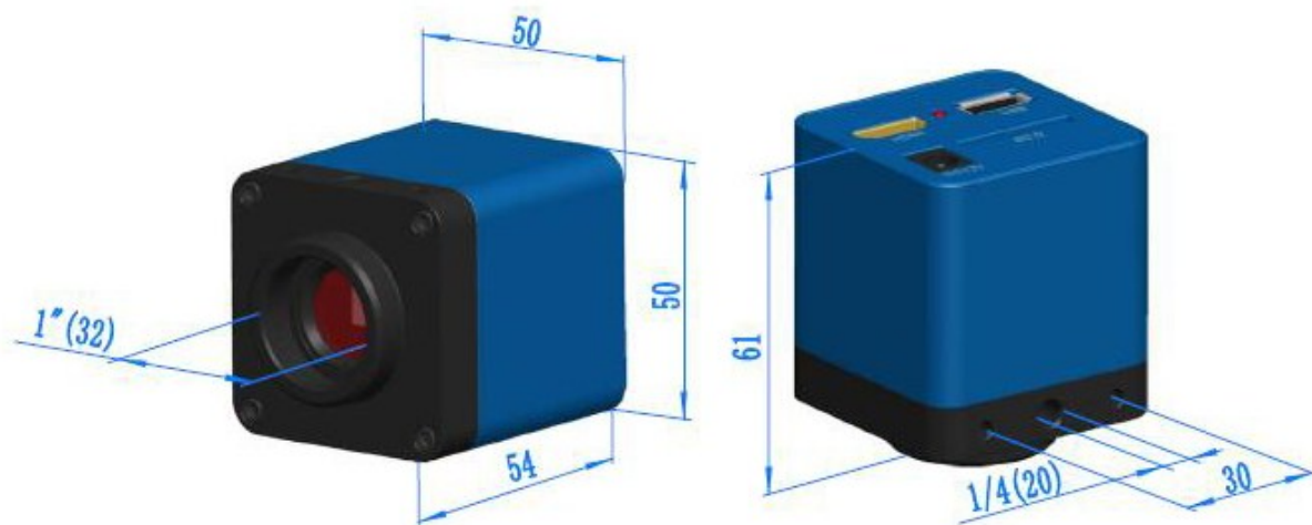
Figure 3-119 Dimension of XCAM720PHC Series Camera
