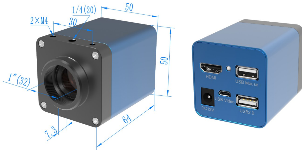
Figure 3-82 XCAMLITE4K-MINI Series Camera's Dimension
