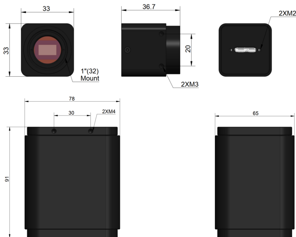
Figure 5-3 Dimension of X5CAM4K_MR Series Camera (Image Capture Sub-device and Master Device)
