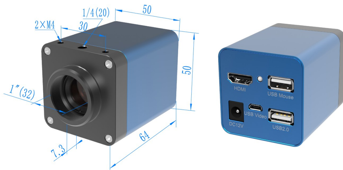
Figure 3-51 Dimension of XCAMTOP4K_MINI Series Camera
