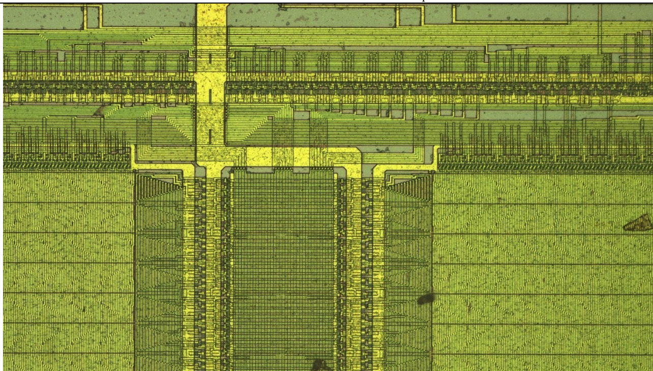
Figure 3-17 Samples Photographed by the SOPTOP RX50M Metallographic Microscopy System Captured with X8CAM4K16MPA
