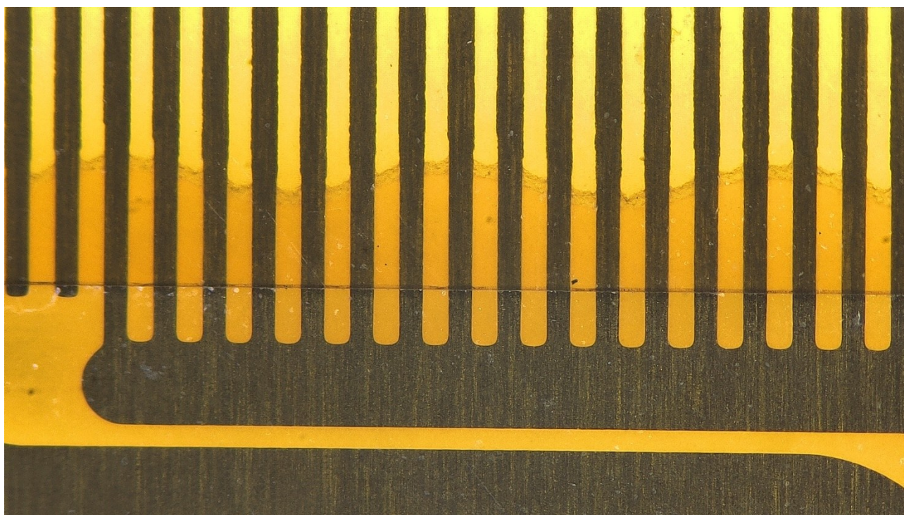
Figure 3-102 FPC line. Captured with O5CAM4K8MPA
