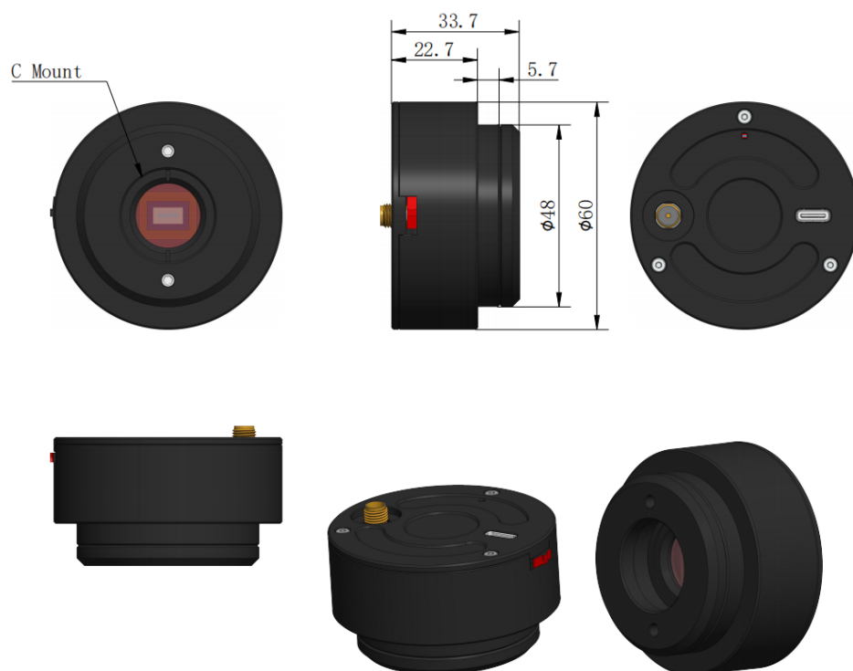
Figure 4-5 Dimension of WUCAM8MPA/WUCAM1080PB Camera
