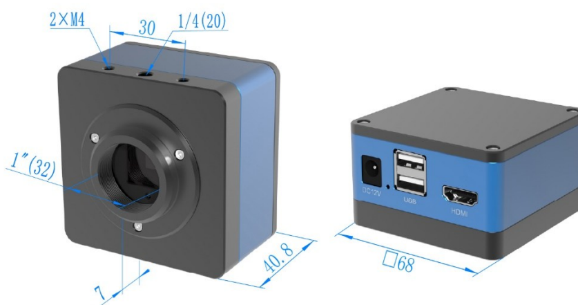
Figure 3-107 Dimension of OCAM Series
