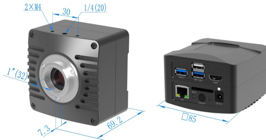
Figure 3-22 Dimension of X7CAM4K Series (Cubic and Flat Shape)
