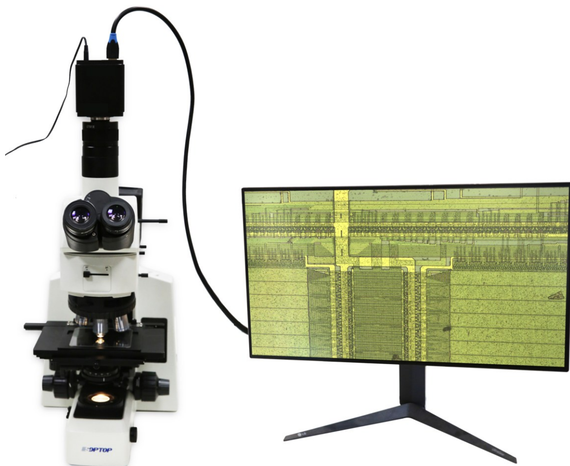
Figure 3-8 X8CAM4K16MPA Camera with Metallographic Microscope
