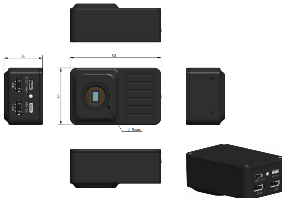
Figure 6-1 Dimension of CXCAM Series
