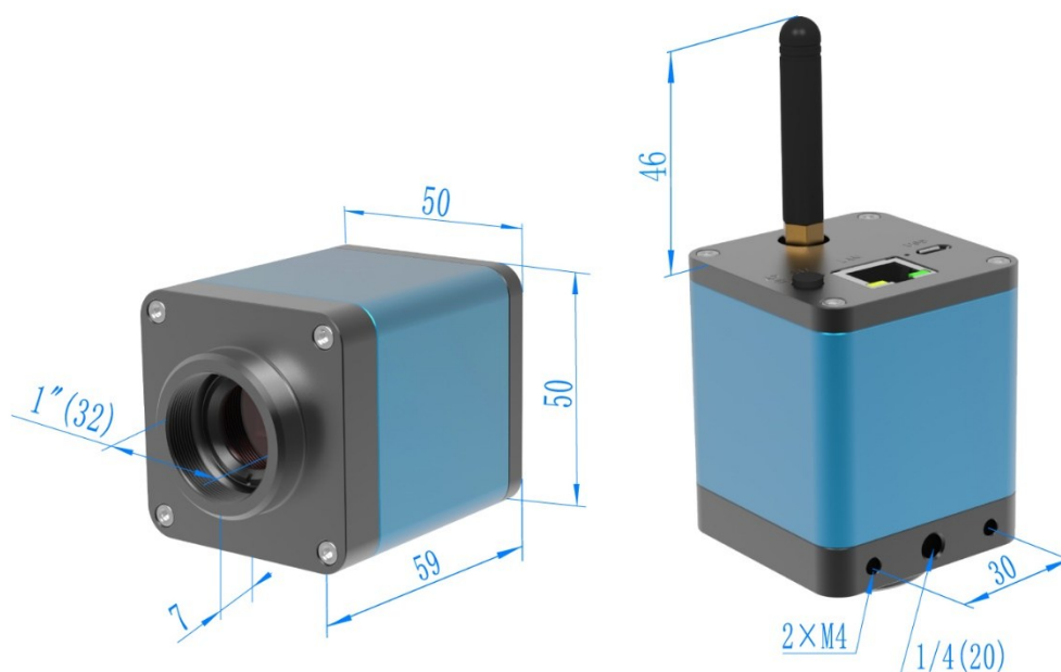
Figure 4-11 Dimension of WEUCAM Series Camera
