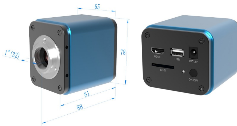
Figure 3-94 Dimension of XCAM1080PHX Series Camera
