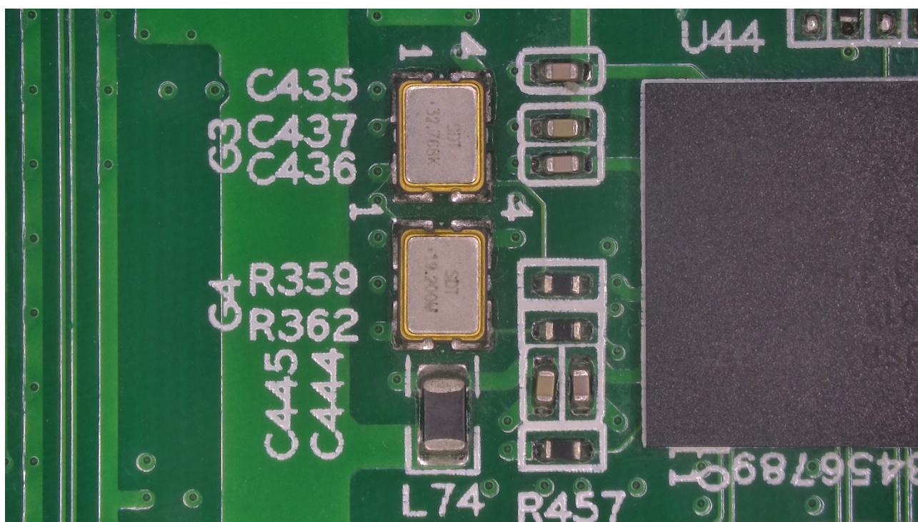
Figure 3-112 Circuit Board Captured with OCAM4K8MPA
