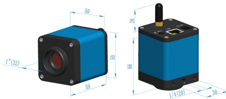
Figure 4-9 Dimension of WECAM Series Camera
