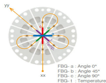
FBG Layout
