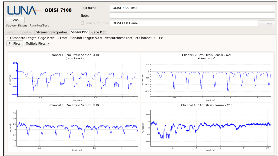
Multichannel sensor plot (strain/temperature versus length) in the ODiSI software.
