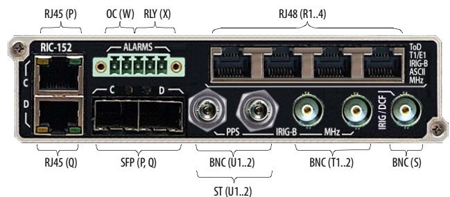
Figure 2. RIC-152 connector layout
