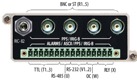
Figure 7. RIC-82 connector layout
