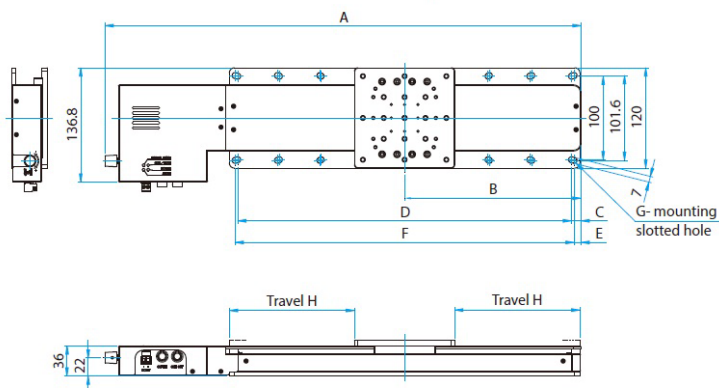
<Mounting hole pattern of a top plate >
