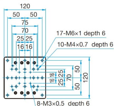
<Mounting hole pattern of a top plate >
