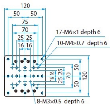
<Mounting hole pattern of a top plate >
